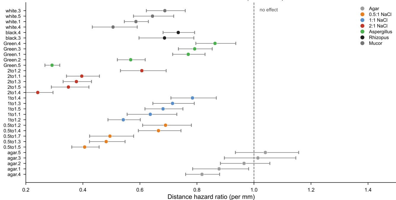
Per-trial Cox PH distance hazard ratio (n = 31 trials)
